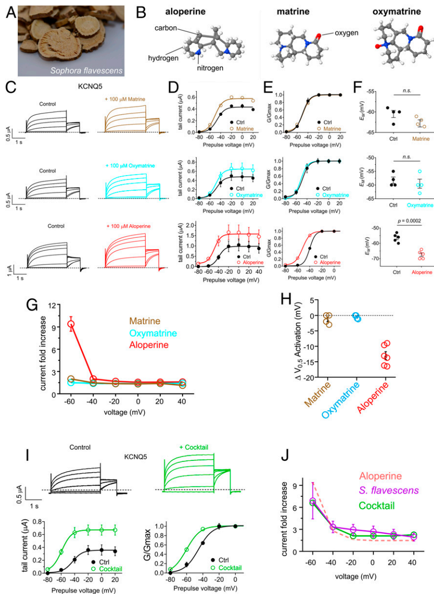
Fig. 2. The S. flavescens alkaloid aloeperine activates KCNQ5. All error bars indicate SEM. (A) Image of dried S. flavescens root slices used in this study. (B) Chemical structures of aloeperine, matrine, and oxymatrine plotted using Jmol. (C) Mean TEVC current traces showing effects of aloeperine, matrine, and oxymatrine (all 100 μM) individually on KCNQ5 expressed in Xenopus oocytes ( n = 4 to 6). (D) Mean tail current versus prepulse voltage relationships for the traces as in C ( n = 4 to 6). (E) Mean normalized tail currents (G/Gmax) versus prepulse voltage relationships for the traces as in C ( n = 4 to 6). (F) Effects of aloeperine, matrine, and oxymatrine (100 μM) individually on resting membrane potential ( E_M ) of undamped oocytes expressing KCNQ5 ( n = 4 to 6). n.s., not statistically significant ( P > 0.05 ). (G) Voltage dependence of effects of aloeperine, matrine, and oxymatrine (100 μM) individually on KCNQ5 (from traces as in C; n = 4 to 6). (H) Mean effects of aloeperine, matrine, and oxymatrine (100 μM) individually on KCNQ5 V_{0.5activation} (from traces as in C; n = 4 to 6). (I) Mean effects of aloeperine, matrine, and oxymatrine (each 1 μM) combined (“Cocktail”) on KCNQ5 expressed in Xenopus oocytes ( n = 5 ). (Upper) Mean TEVC traces; (Lower Left) mean tail current versus prepulse voltage relationships; (Lower Right) mean normalized tail currents (G/Gmax) versus prepulse voltage relationships. (J) Comparison of effects of aloeperine (100 μM), cocktail, and S. flavescens extract (1%) on KCNQ5 activity, quantified as current fold change versus voltage ( n = 5 to 6).
