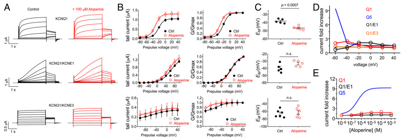
Fig. 5. Aloperine weakly activates homomeric KCNQ1 but not KCNQ1-KCNE complexes. All error bars indicate SEM. (A) Mean TEVC current traces showing effects of aloperine (100 \mu M) on KCNQ1, KCNQ1/KCNE1, and KCNQ1/KCNE3 channels expressed in Xenopus oocytes ( n = 5 to 6). (B) Mean tail current (Left) and mean normalized tail currents ( G/G_{max} ; Right) versus prepulse voltage relationships for the traces as in A ( n = 5 to 6). (C) Effects of aloperine (100 \mu M) on resting membrane potential ( E_M ) of unclamped oocytes expressing channels as in A ( n = 5 to 6). n.s., not statistically significant ( P > 0.05 ). (D) Voltage dependence of effects of aloperine (100 \mu M) on channels indicated (from traces as in A; n = 5 to 6). (E) Aloperine dose response calculated from fold increase in current at -60 mV for channels as indicated ( n = 5 to 6).
