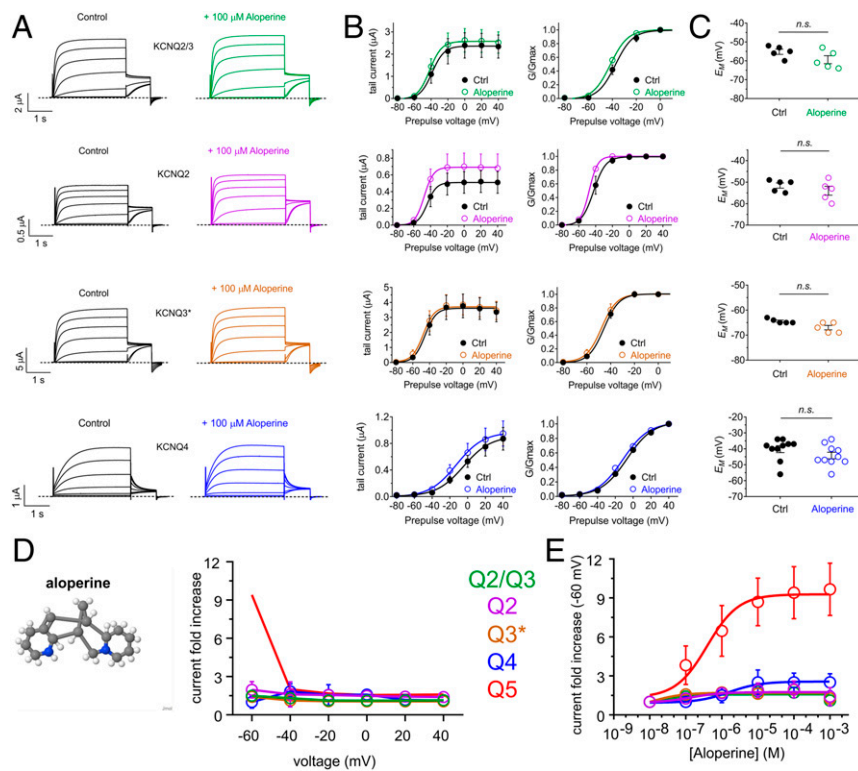
Fig. 4. Aloperine is a potent and selective activator of KCNQ5 channels. All error bars indicate SEM. (A) Mean TEVC current traces showing effects of aloperine (100 \mu M) on KCNQ2/3 and homomeric KCNQ2, KCNQ3*, and KCNQ4 expressed in Xenopus oocytes ( n = 5 to 10). (B) Mean tail current (Left) and mean normalized tail currents ( G/G_{max} ; Right) versus prepulse voltage relationships for the traces as in A ( n = 5 to 10). (C) Effects of aloperine (100 \mu M) on resting membrane potential ( E_M ) of unclamped oocytes expressing channels as in A ( n = 5 to 10). n.s., not statistically significant ( P > 0.05 ). (D) Voltage dependence of effects of aloperine (100 \mu M) on channels indicated (from traces as in A; n = 5 to 10). (E) Aloperine dose response calculated from fold increase in current at -60 mV for channels as indicated ( n = 5 to 10).
